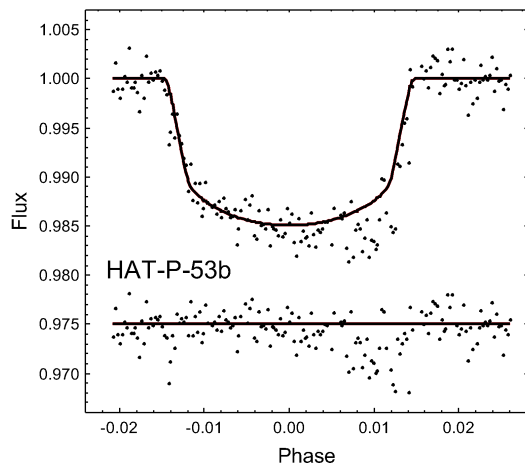
Fig. 1. Top: the Rozhen transit of HAT-P-53b and the synthetic curve corresponding to the best solution; bottom: the residuals of the fit. The observational data are accessible in the form of tables (whose samples A1 and A2 are shown in Appendix) at www.irida-observatory.org/Observations/exo-HAT-P-53andXO-5b.rar .
