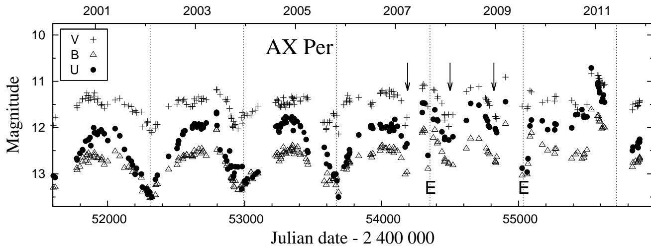
Fig. 16 The UBV light curves of AX Per from 2000 to the present. New observations (Table 16) are from 2007.2. Vertical dotted lines denote positions of eclipses according to their ephemeris (5) and arrows denote the minima of a wave that appeared in the LC during the 2007-10 active phase.
