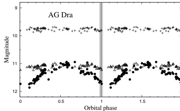
Fig. 14 Phase diagram of the UBV measurements during the current quiescent phase from 2008 February 24 to our last observation on 2011 November 18 (Table 13). The width of the grey band represents uncertainties in the position of the inferior conjunction of the giant as given by elements of Fekel et al. (2000).
