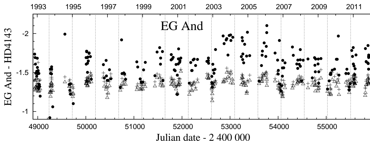
Fig. 1 \Delta U(\bullet) , \Delta B(\triangle) , \Delta V(+) light curves of EG And from 1993. Vertical dotted lines mark times of the inferior conjunction of the giant according to the ephemeris (1). Data are from Table 2 and previous papers of this series (see Paper I and references therein).
