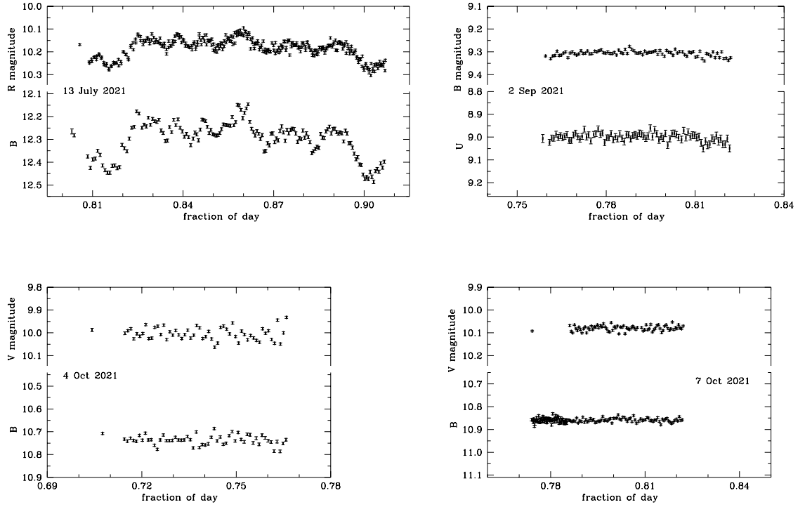
Figure 1: Flickering of RS Oph before and the cessation of it after the 2021 outburst.
