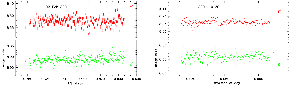
Figure 1: Search for flickering of MWC 560.
