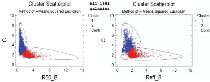
Figure 4. Cluster analysis of: Radius containing 50% of the flux R_{50} and the Effective radius R_{\text{eff}} against the Index of Concentration distribution.
