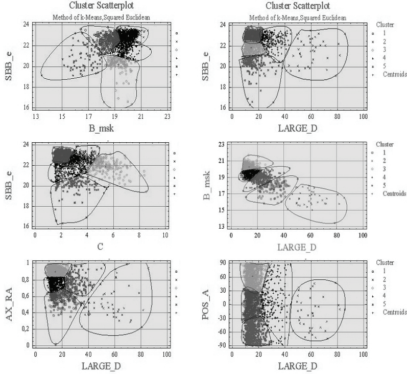
Figure 2. Cluster analysis of: Surface Brightness SBB_{eff} against Total magnitude B_{msk} , Index of Concentration C and diameters Large\_D and of Large diameters Large\_D against Total magnitude B_{msk} , Axis ratio AX\_RA and position angle Pos\_A .
