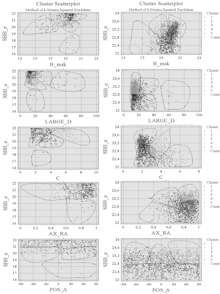
Figure 3. Clustering SBB_{eff} , B_{msk} , C and Large\_D for: Right panel - HSBG, Left panel - LSBG.
