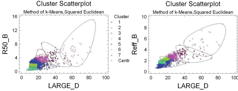
Figure 5. Cluster analysis – looking for probably AGN. The members of cluster 7 are potentially candidates for AGNs.
