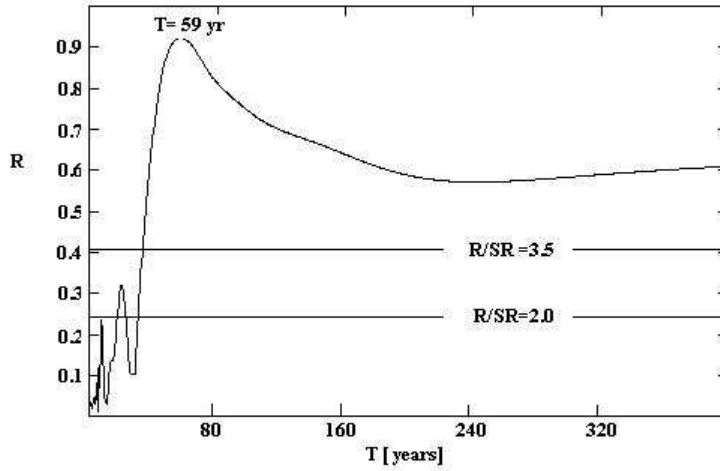
Fig. 5. The T - R spectra of the Group sunspot number (11-yr smoothing annual values; AD 1913-1979).
