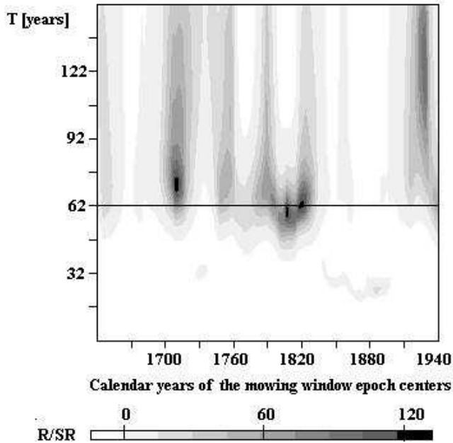
Fig. 6. The T - R spectra evolution of the 11 year smoothed GSN data in the range of periods 2; T \leq 152 years. By the horizontal line at T=62 years the typical duration of the subcentennial cycle is signed. The most white areas on the map to statistically non-significant values of -0.11 \leq R/\sigma R \leq 0 are corresponded.
