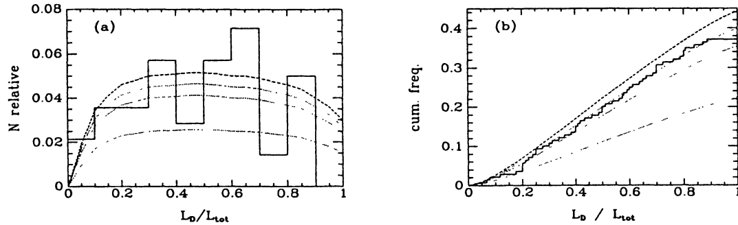
Fig. 12. Relative (a) and cumulative (b) frequency for the relative disk luminosities. Solid line – determinations from the \epsilon_{21.85} - \langle c_4 \rangle diagram. The distribution has been normalized with the total number of galaxies fainter than m_T = 12^m 7 . Dashed line – model prediction for a uniform intrinsic distribution, corrected for the incompleteness due to the limits enforced on \epsilon_{21.85} and \langle c_4 \rangle . Dotted lines – model predictions for a uniform intrinsic distribution plus a fraction of diskless galaxies. Models for fractions of 0.1, 0.2, and 0.5 are shown. A higher fraction of diskless galaxies moves the curve for the normalized distribution downwards in both (a) and (b). (From JF94).
