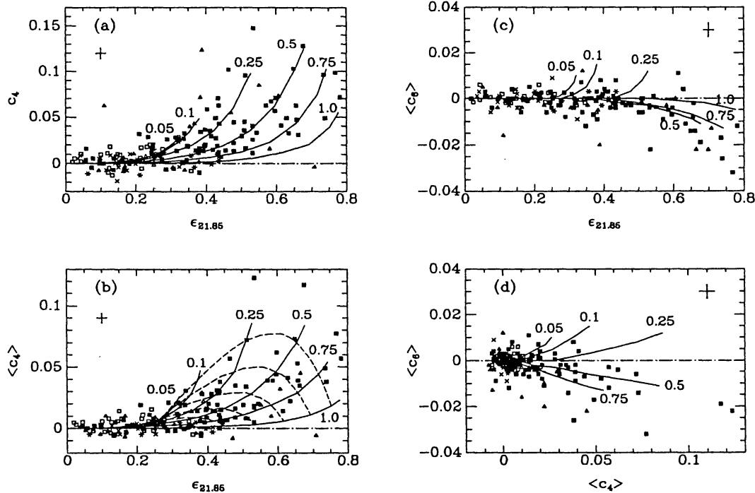
Fig. 11. Fourth and 6th order Fourier coefficients plotted against ellipticity and versus each other. Data symbols as in Figure 9. Galaxies with uncertainty on c_4 respectively \langle c_4 \rangle larger than 0.02 are not plotted. Typical measurement errors are given on the panels. The models with a_{eB} = a_{eD} are overplotted. The curves are labeled with L_D/L_{tot} . The dashed lines on (b) mark the inclinations where \cos i = 0.1, 0.2, 0.3, 0.4 and 0.5 (i.e. i = 84^\circ, 78^\circ, 73^\circ, 66^\circ , and 60^\circ ), from top to bottom. No dashed line is shown for the i = 90^\circ (i.e. edge-on) models, but this line would be above the i = 84^\circ dashed line, connecting the end points of the solid lines. It is seen that for a given L_D/L_{tot} the highest inclination gives the largest \langle c_4 \rangle . The non-zero coefficients for the pure disk-model are due to the inclusion of seeing effects in the models. (From JF94.)
